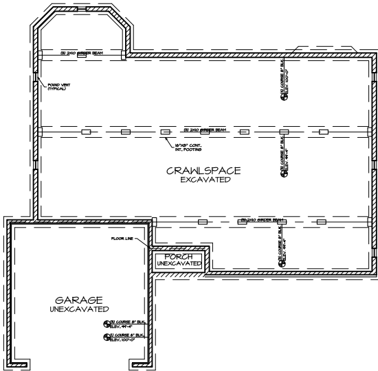
1 FOUNDATION PLAN A-2
